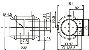
TD-160/100 N SILENT
